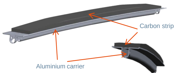
Main pantograph strip Reference 3-54201
