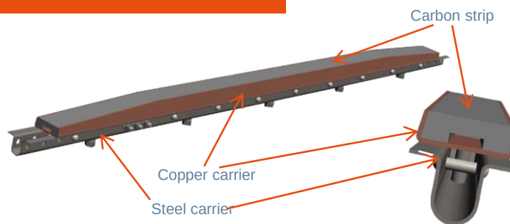
Frost resistant strip Reference 3-39579
